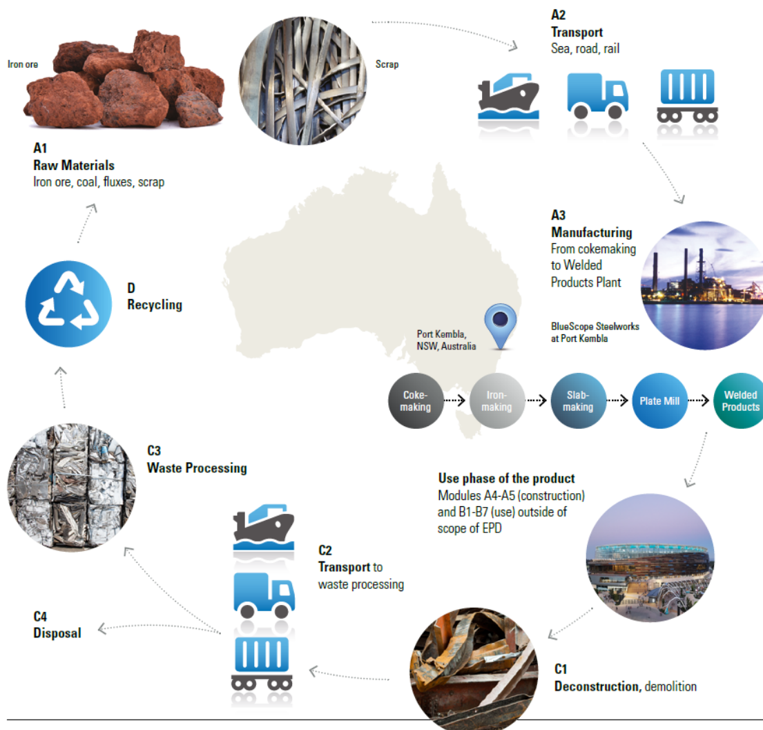
Figure 1 – Welded Beams and Columns manufacturing process and life cycle stages
